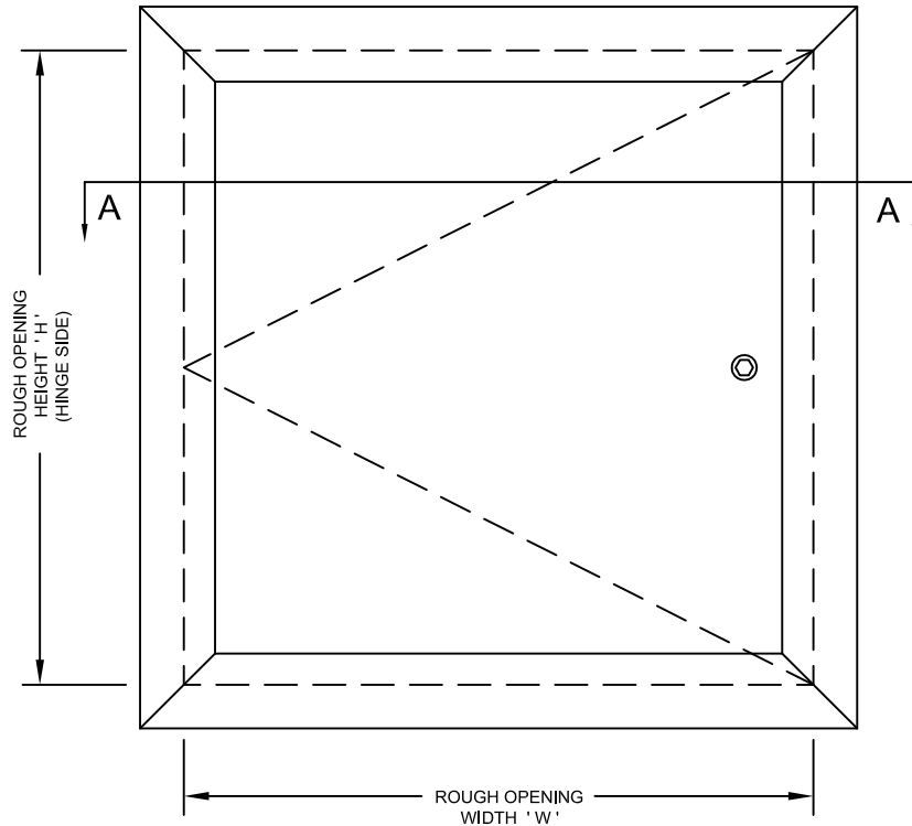
FRONT ELEVATION
