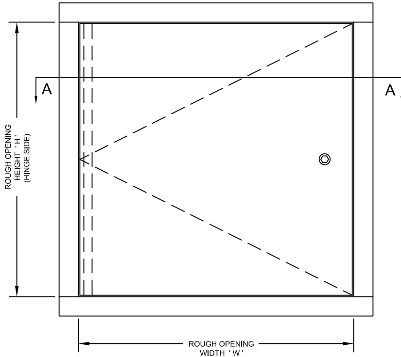
FRONT ELEVATION
