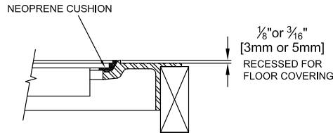
FLANGE DETAIL
