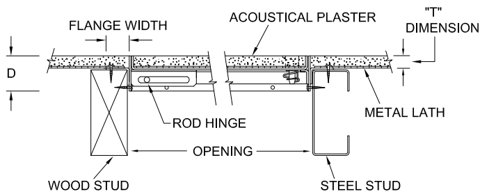
Concealed Rod Hinge
