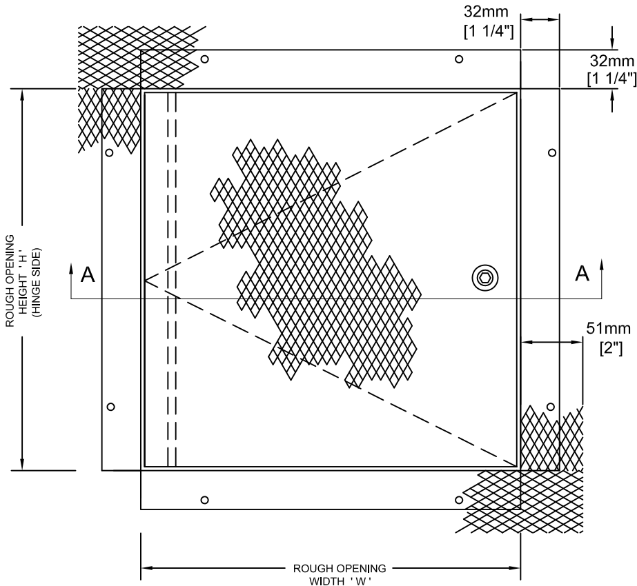
FRONT ELEVATION
