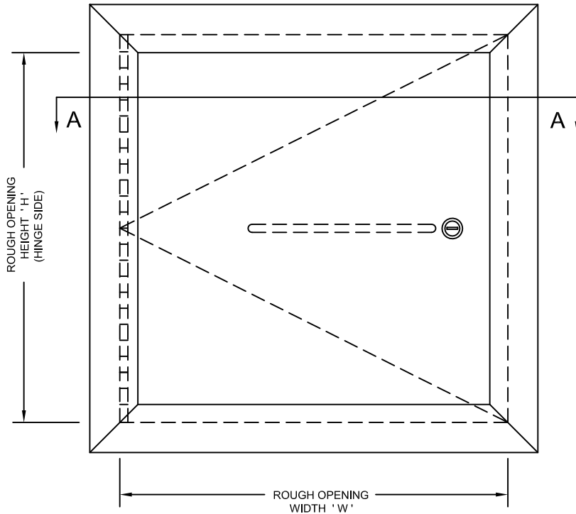
FRONT ELEVATION
