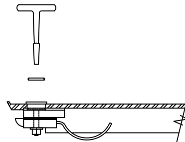
SPRING LATCH ASSEMBLY DETAIL
