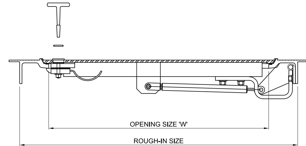
DOOR IN CLOSED POSITION
