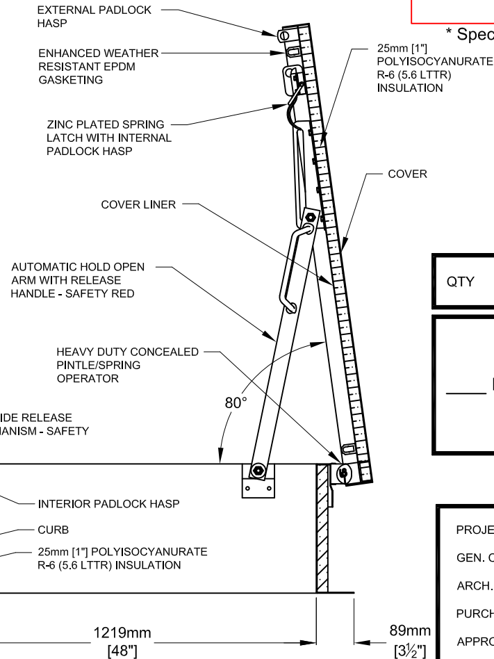
SECTION
