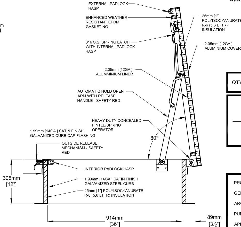
SECTION
